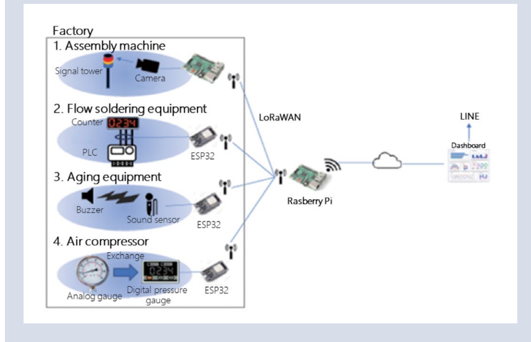
FIGURE 5-11 EXAMPLE OF A SYSTEM CONFIGURATION DIAGRAM
