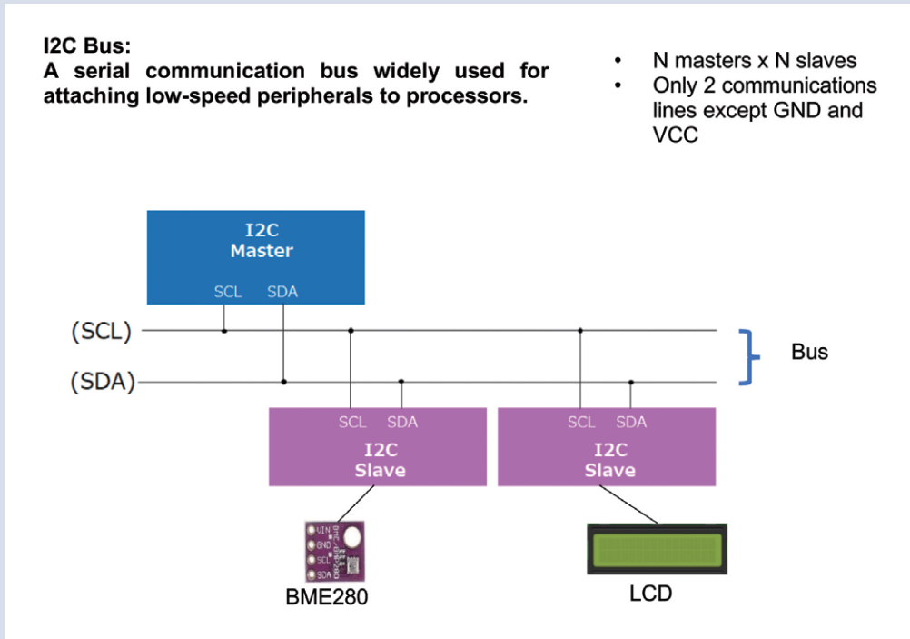
I2C INTERFACE [76]
