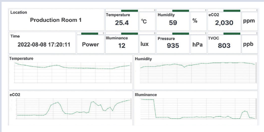
FIGURE 3-23 DASHBOARD (DETAIL)
