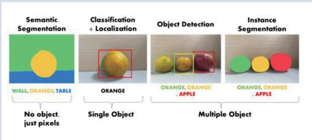
FIGURE 2-21 MAJOR TASKS OF MACHINE VISION
