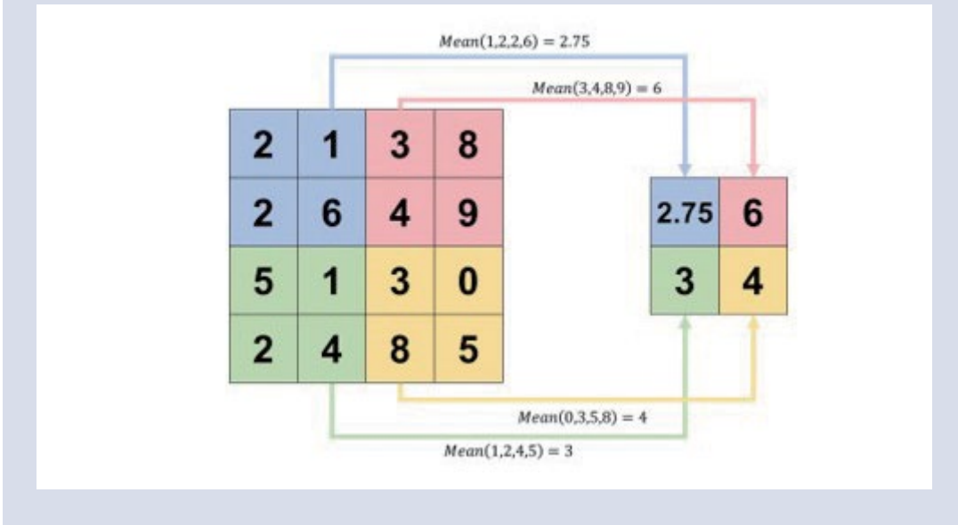
FIGURE 2-26 THE OPERATION OF MEAN POOLING
