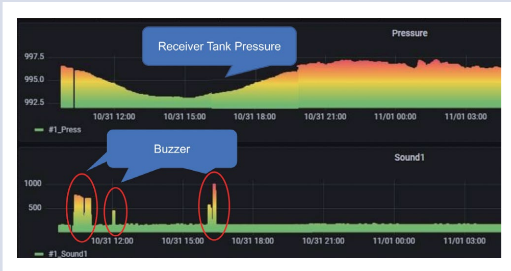
FIGURE 3-6 RECEIVER TANK PRESSURE AND AGING FURNACE ALARM
